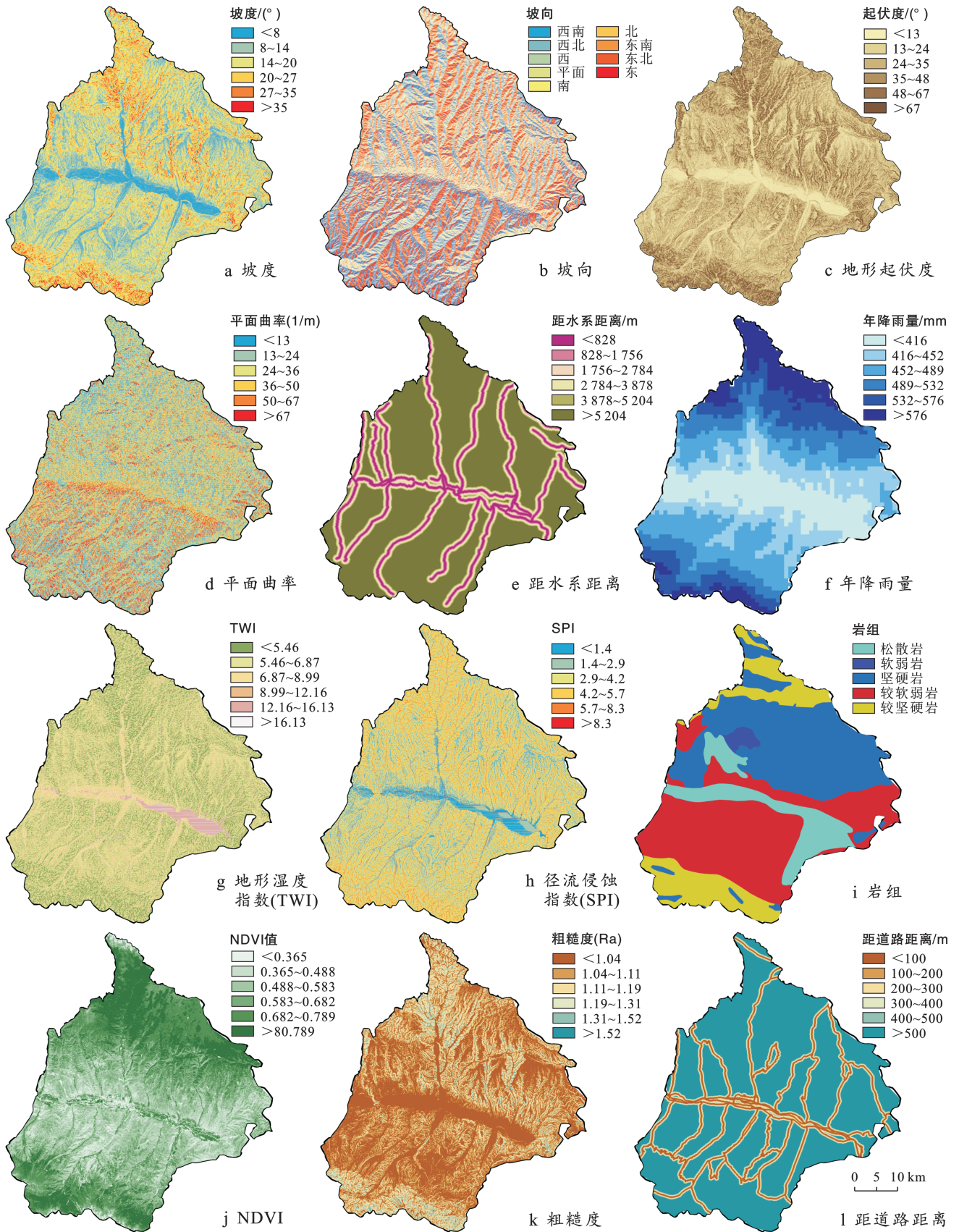
图4 乐都区滑坡影响因子 Fig.4 Landslide influencing factors of Ledu District
